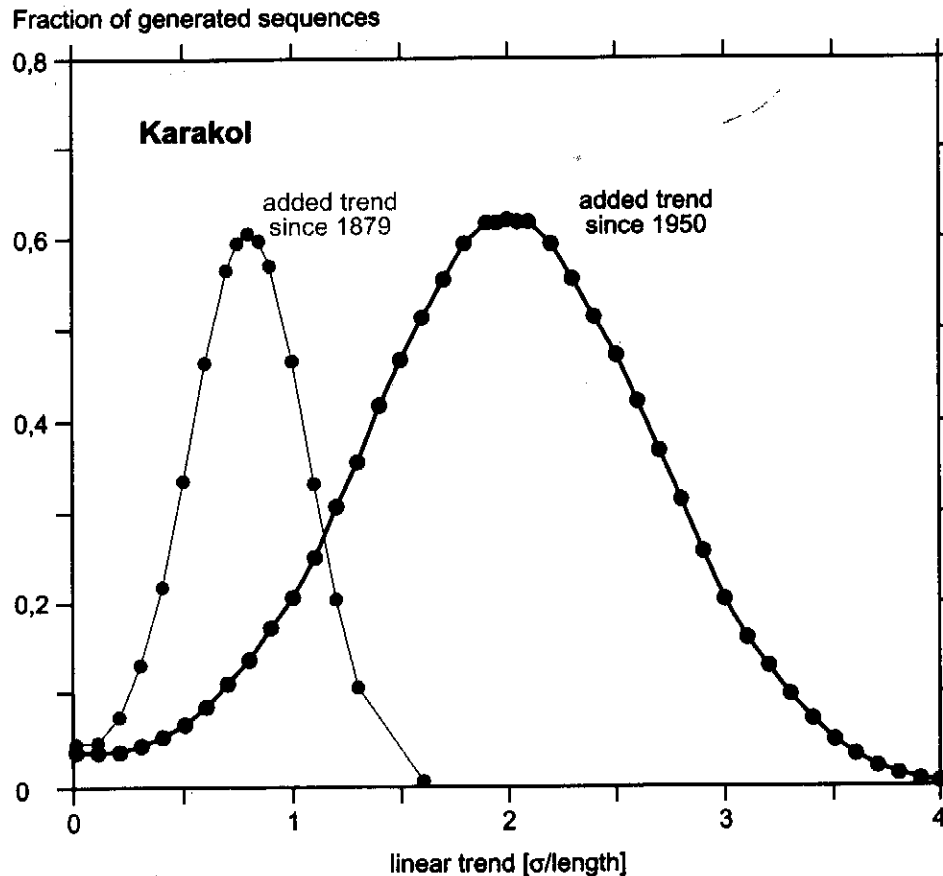
Fig. 8: Fraction of simulated random sequences, which provide comparable exponents, as does the temperature series of Karakol, for the FA as well as for the DFA, depending on the strength of an added trend since 1950 (Karakol: \alpha_{\text{DFA2}} = 0.66 \pm 0.05 ; \alpha_{\text{FA}} = 0.77 \pm 0.05 )
